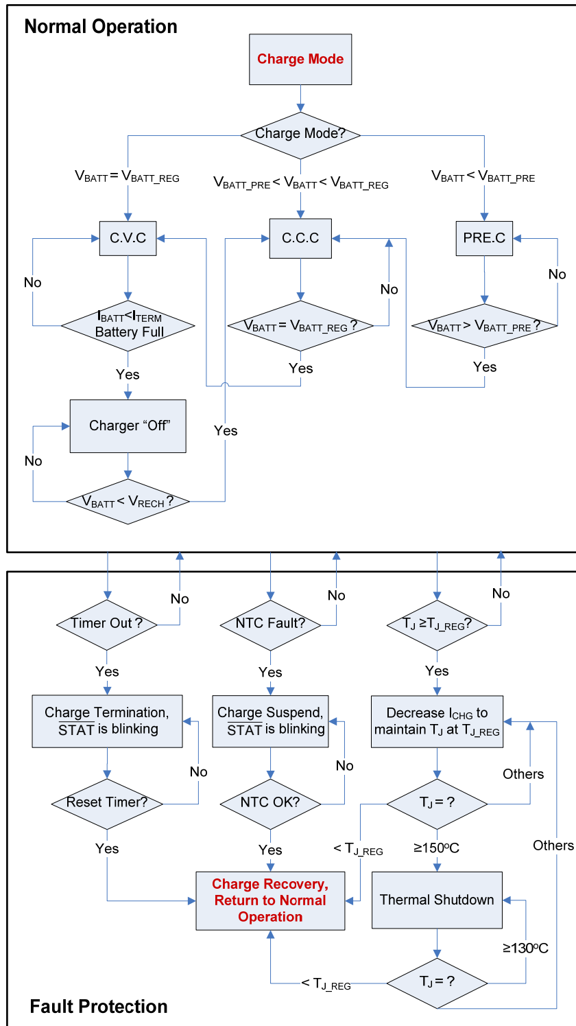
Figure 6: Charging Process
