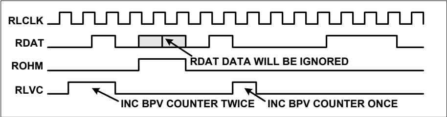
Figure 8-8. RX Line I/O UNI Octet Aligned OHM Functional Timing Diagram
