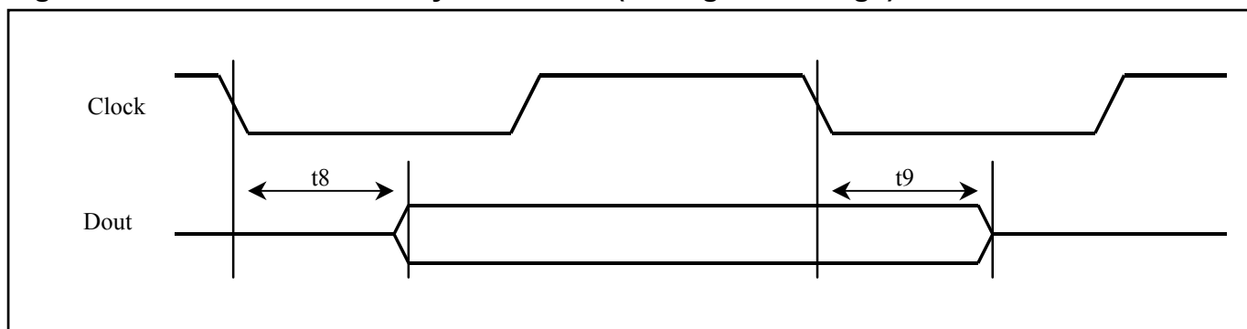
Figure 18-6. To/From Hi-Z Delay Definitions (Falling Clock Edge)
