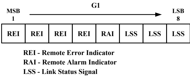
Figure 10-31. DS3 PLCP G1 Byte Format
