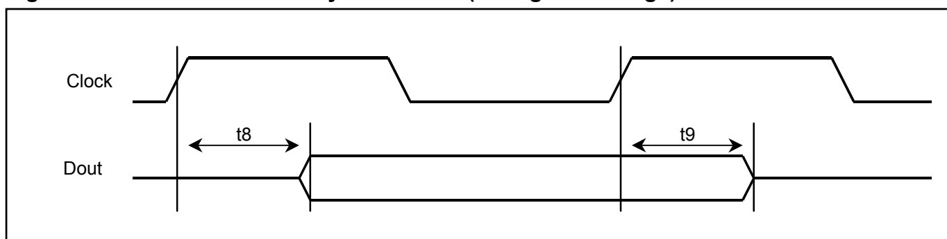
Figure 18-5. To/From Hi-Z Delay Definitions (Rising Clock Edge)
