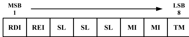
Figure 10-43. MA Byte Format
