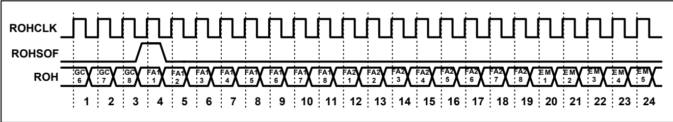
Figure 8-11. E3 G.832 Framing Receive Overhead Port Timing
