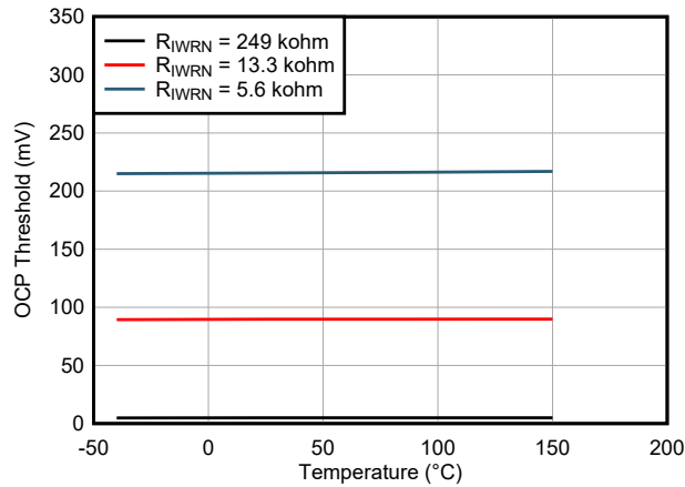
Figure 7-7. Overcurrent Threshold ( V_{SNS\_WRN} ) vs Temperature
