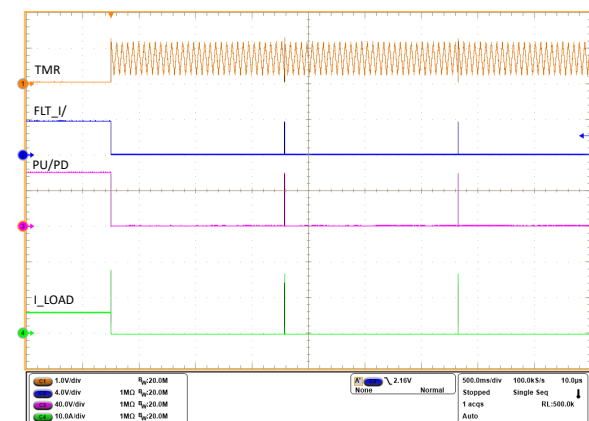
Figure 10-10. Auto-Retry Response of TPS4811-Q1 for an Overcurrent Fault
