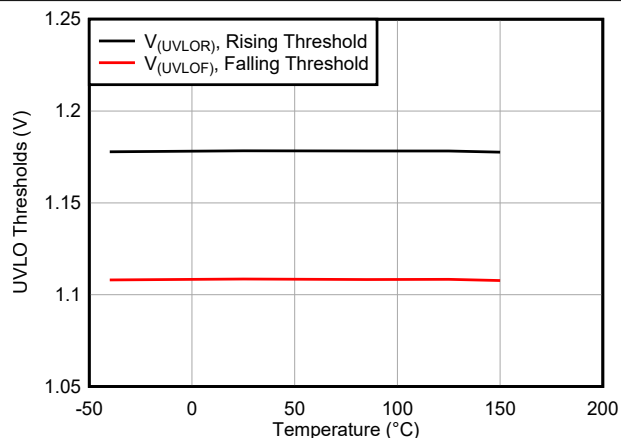
Figure 7-14. Input Supply UVLO Thresholds vs Temperature
