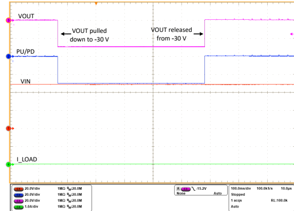
Figure 9-16. Output Short to -30 V Response with VIN = 48 V and INP = LOW
