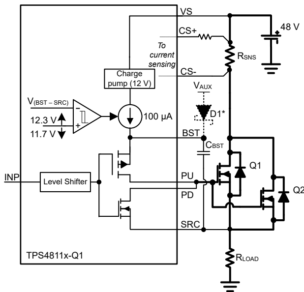
Figure 9-3. Gate Driver
