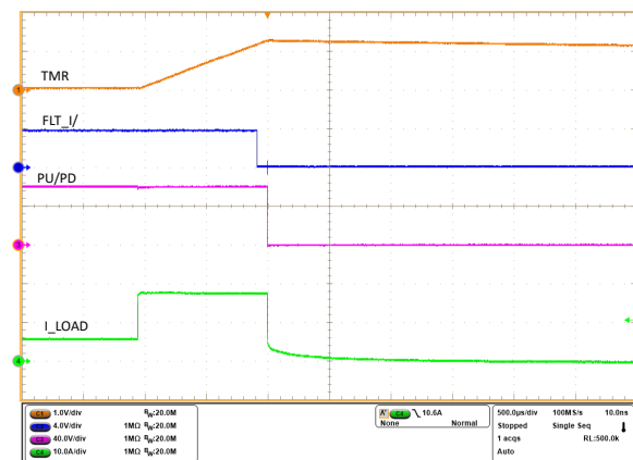
Figure 10-9. Overcurrent Response of TPS4811-Q1 for a Load Step from 5 A to 18 A With 15-A Overcurrent Protection Setting
