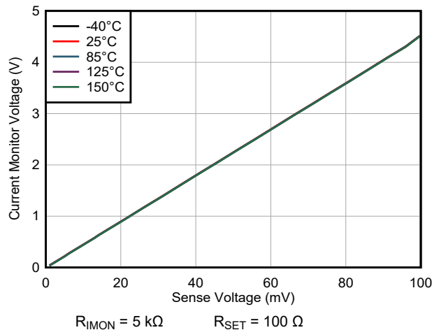
Figure 7-9. Current Monitor Output ( V_{IMON} ) vs Sense Voltage ( V_{SNS} )
