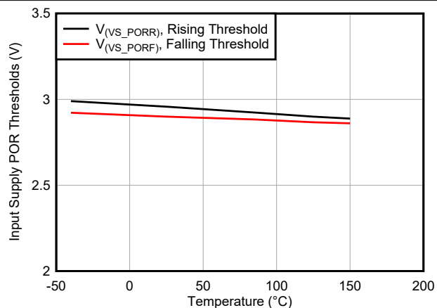
Figure 7-13. Input Supply POR Thresholds vs Temperature
