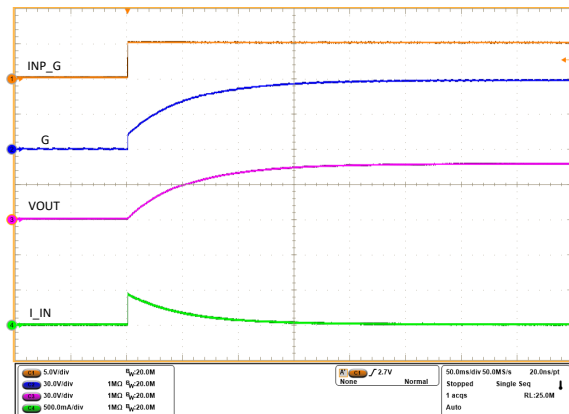
Figure 10-15. Pre-charge Profile of the Output Capacitance (VIN = 48 V, C OUT = 440 \mu F, No Load)
