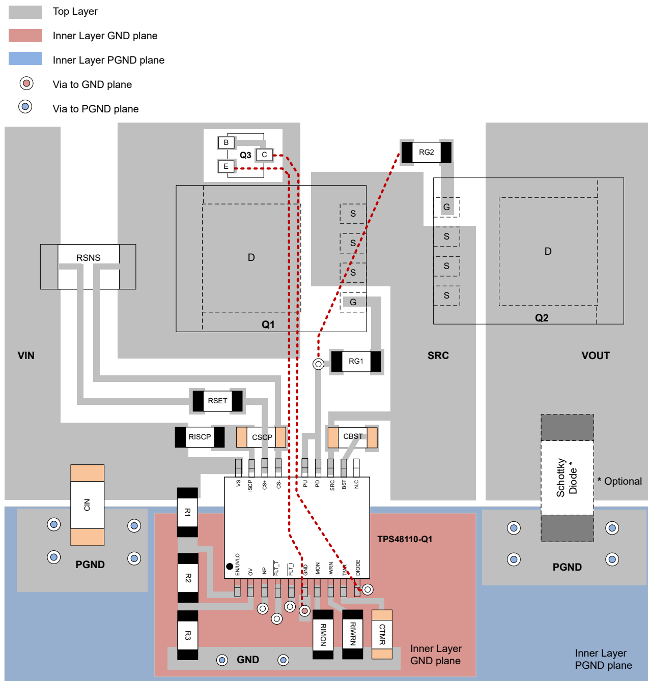
Figure 10-19. Typical PCB Layout Example With TPS4811-Q1 With B2B MOSFETs
