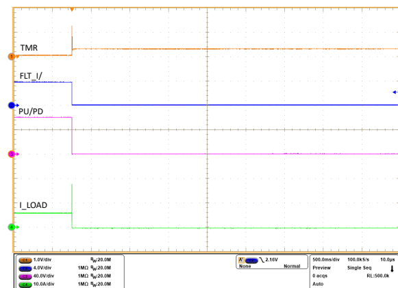
Figure 10-11. Latch-off Response of TPS4811-Q1 for an Overcurrent Fault
