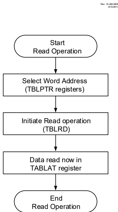
Figure 11-5. Program Flash Memory Read Flowchart
