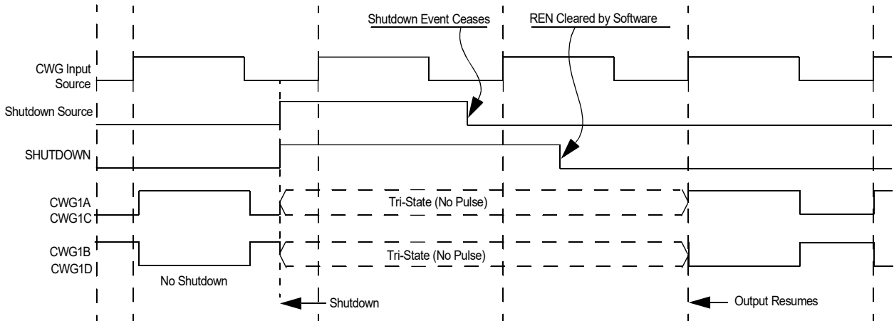
Figure 24-15. SHUTDOWN FUNCTIONALITY, AUTO-RESTART DISABLED (REN = 0, LSAC = 01, LSBD = 01)
