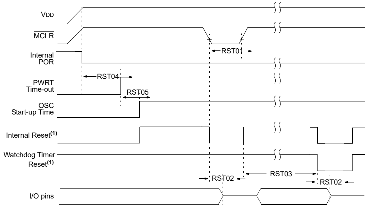
Figure 38-8. Reset, Watchdog Timer, Oscillator Start-up Time and Power-up Timer Timing
