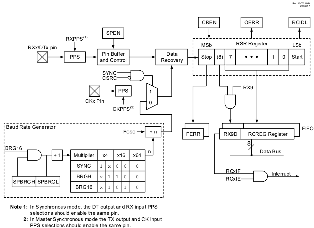
Figure 27-2. EUSART Receive Block Diagram
