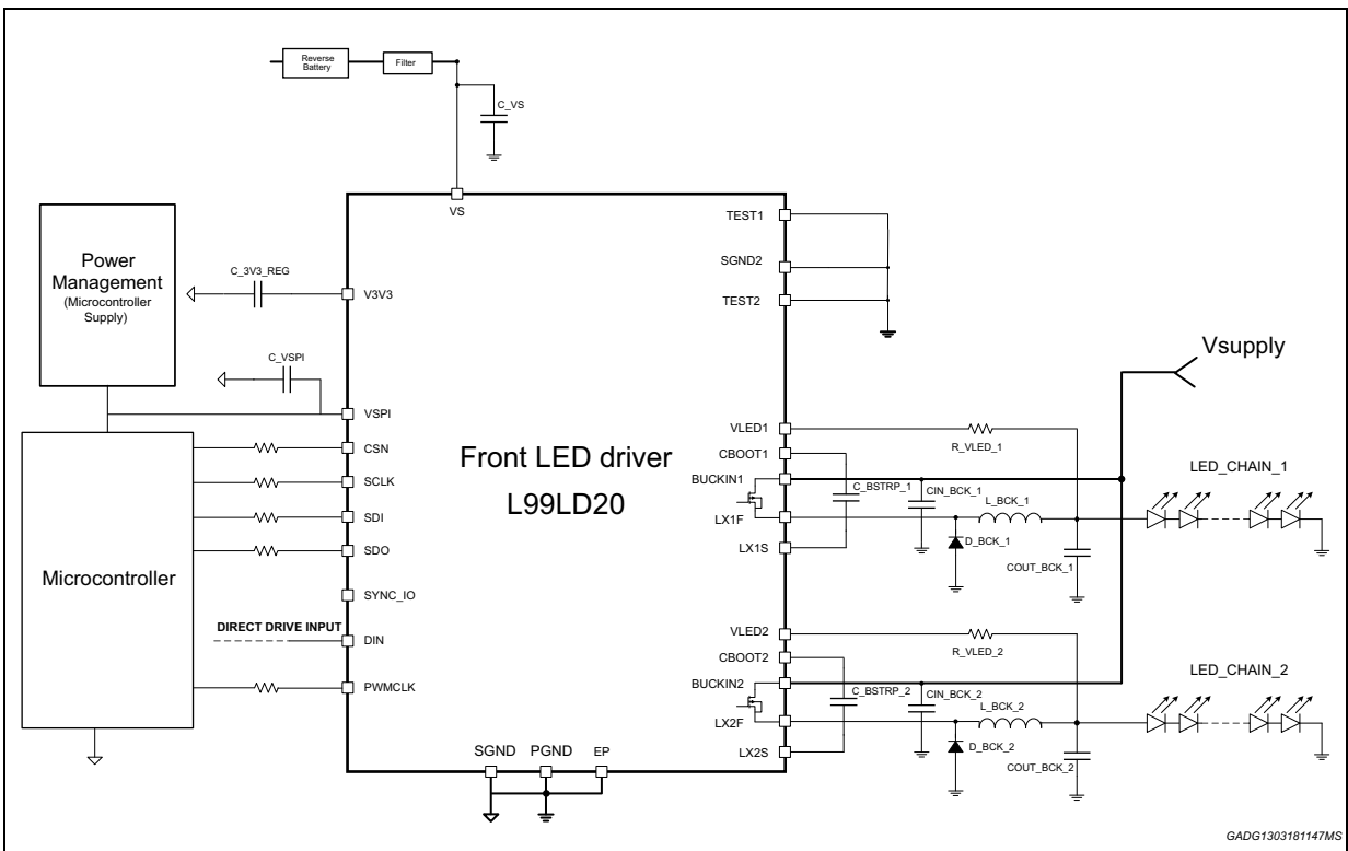
Figure 3. Application diagram
