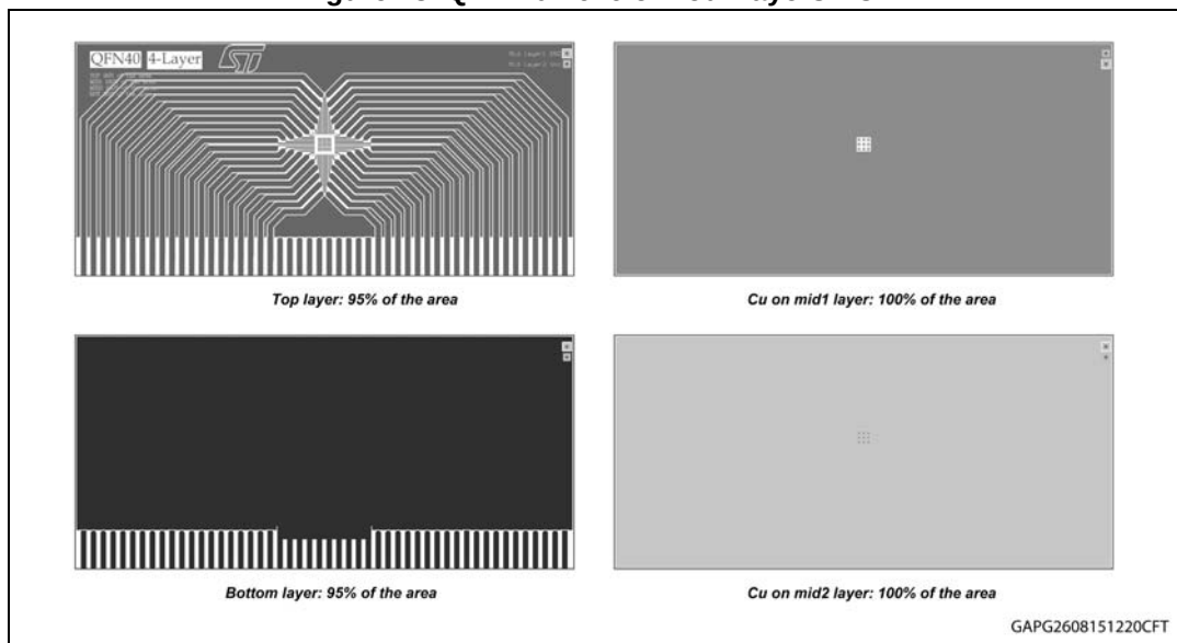
Figure 13. QFN-40L 6x6 on four-layers PCB
