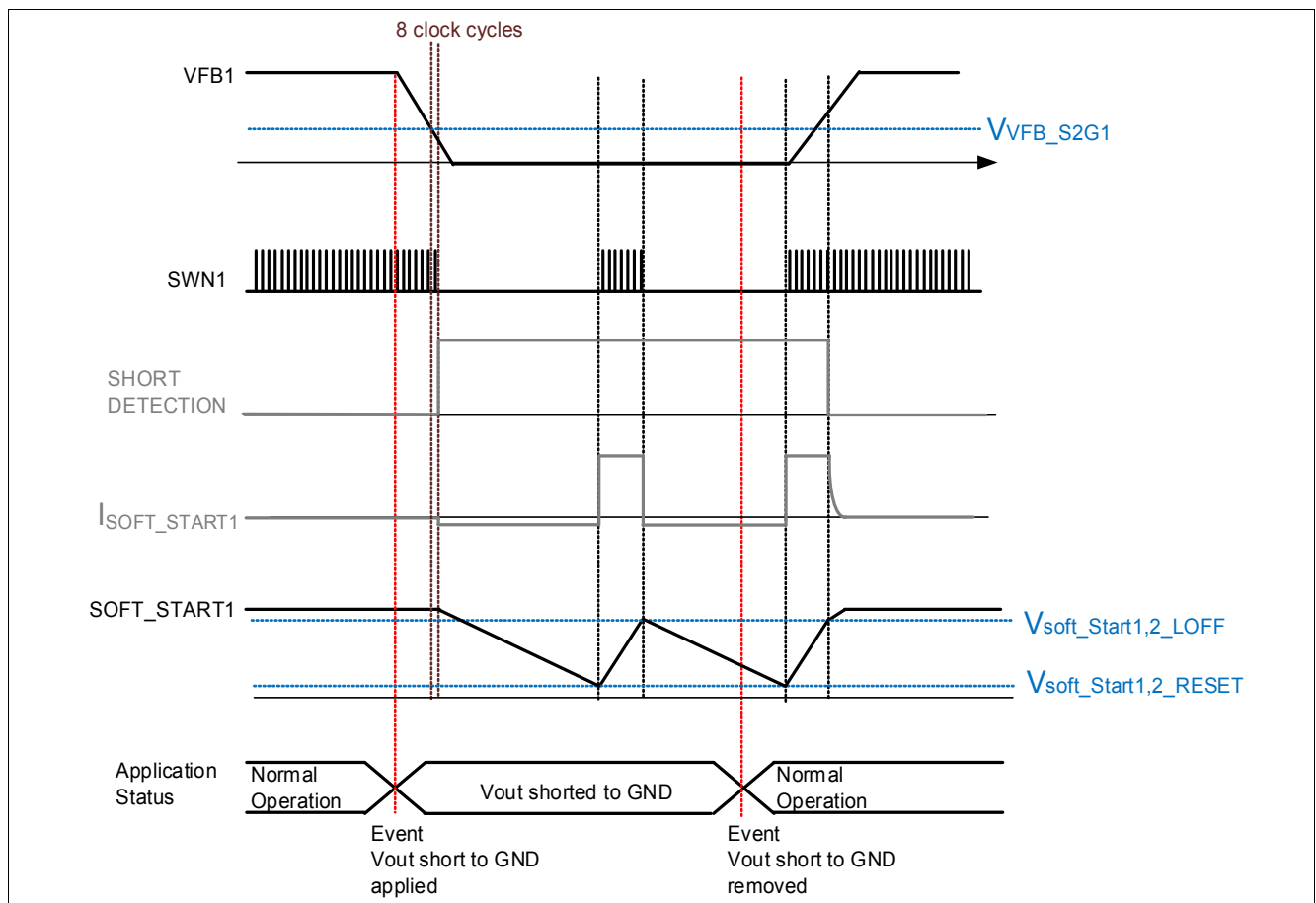
Figure 8 Soft Start timing diagram on a short to ground detected by the VFB1 pin
