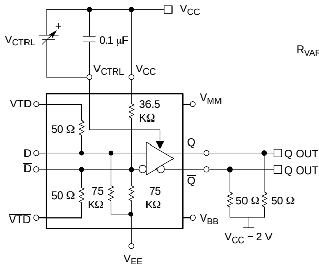
Figure 2. Logic Diagram/ Voltage Source Implementation
