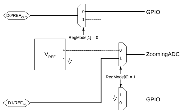
Figure 15 - D0 is Digital Input / Output and D1 is Reference Voltage Input
