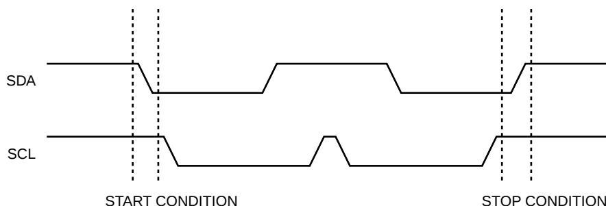
Figure 3. Start/Stop Condition
