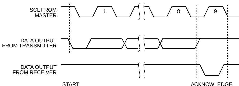
Figure 4. Acknowledge Condition
