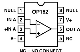
8-Lead Plastic DIP (P Suffix)
