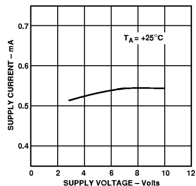
Figure 12. OP462 Supply Current/Amplifier vs. Supply Voltage
