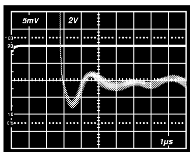
Figure 43. Negative Slope Settling Time
