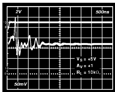
Figure 32. Oscilloscope Photo of V_S and V_{OUT}
