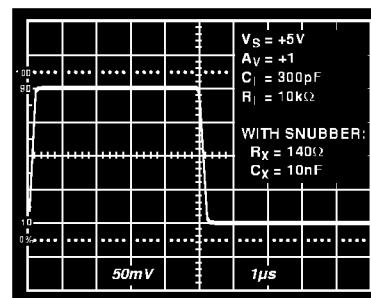
Figure 36. A Photo of a Nice Square Wave at the Output
