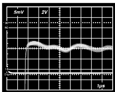
Figure 42. Positive Slope Settling Time
