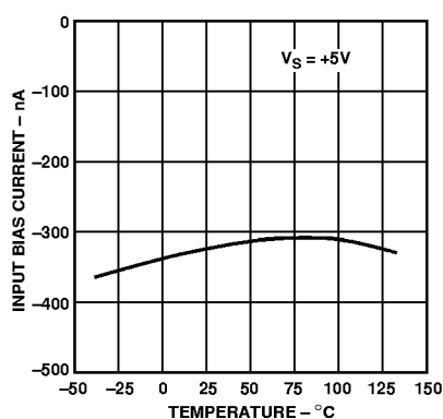
Figure 5. OP462 Input Bias Current vs. Temperature
