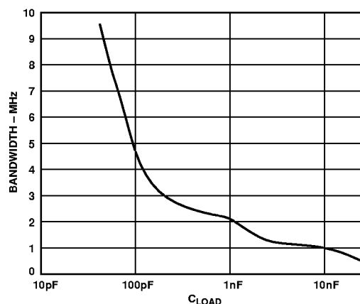
Figure 37. Unity Gain Bandwidth vs. C_{LOAD}
