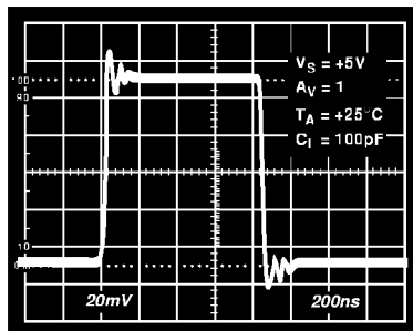
Figure 25. Small Signal Transient Response
