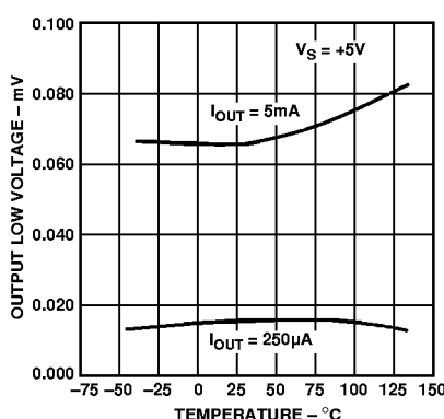
Figure 8. OP462 Output Low Voltage vs. Temperature
