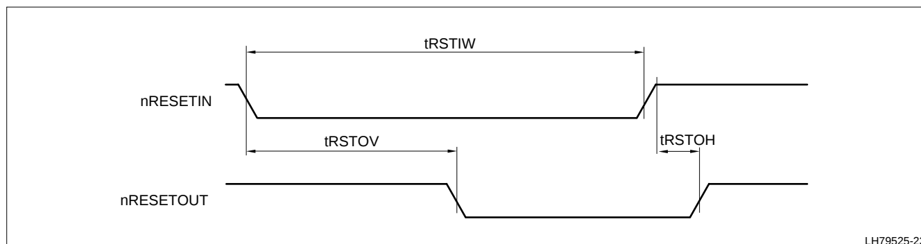
Figure 38. External Reset
