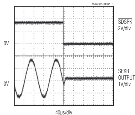
SHUTDOWN RESPONSE
