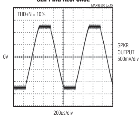
CLIPPING RESPONSE
