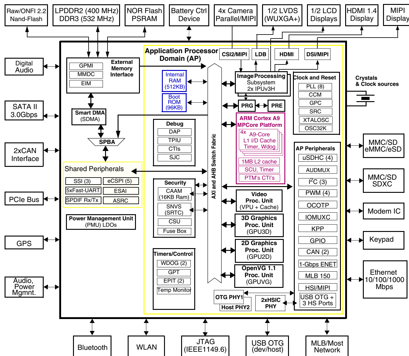
Figure 2. i.MX 6DualPlus/6QuadPlus Consumer Grade System Block Diagram
