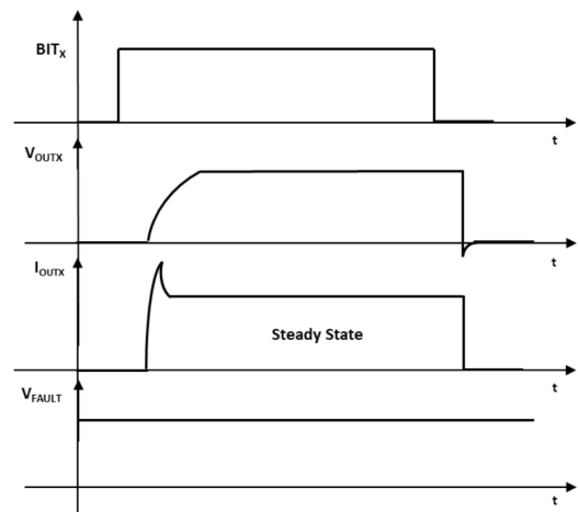
Figure 17. Switching on bulb lamp
