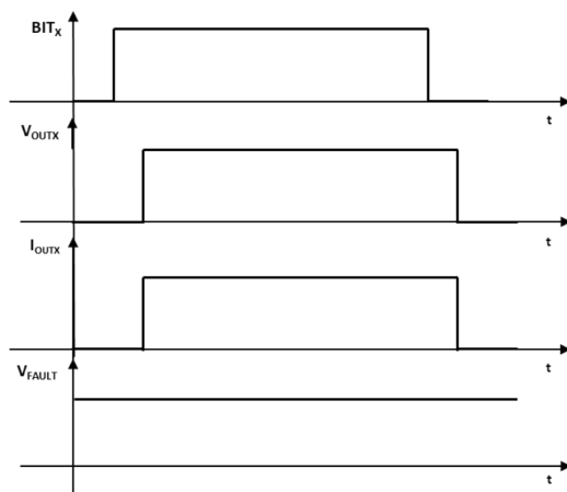
Figure 16. Switching on resistive load
