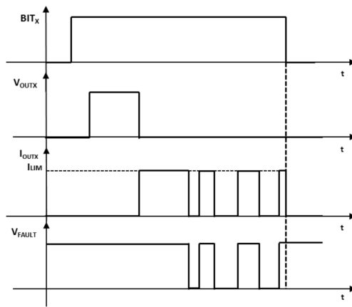
Figure 20. Short-circuit (with OVT) during ON-state
