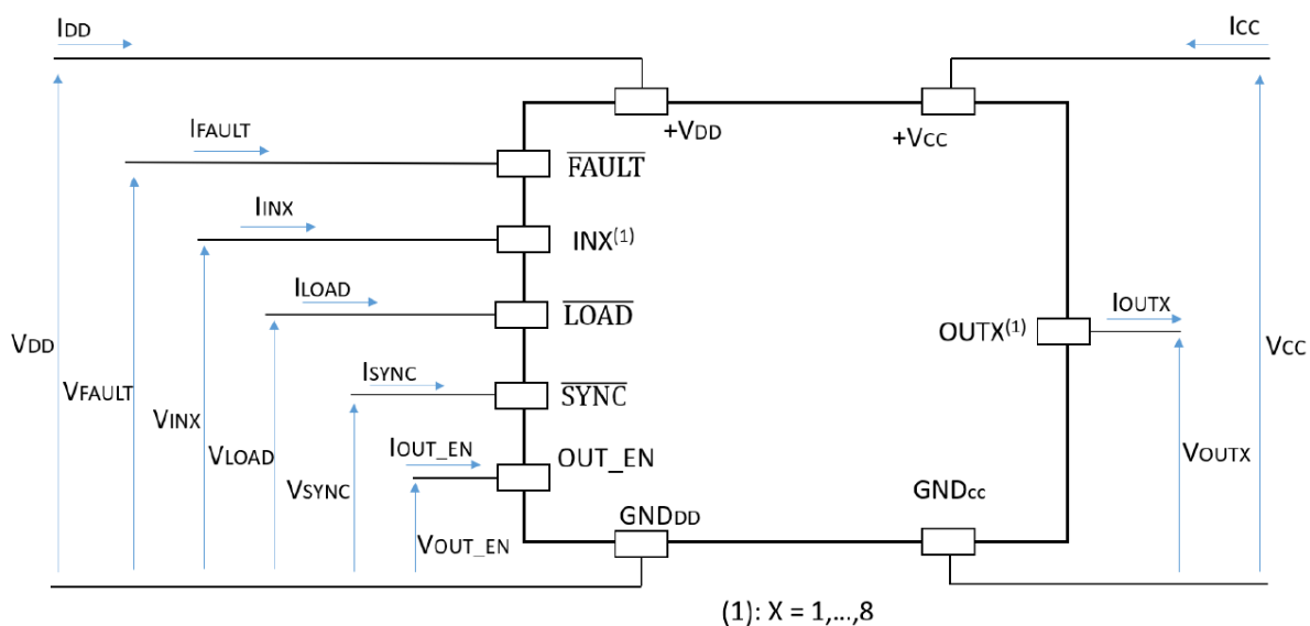
Figure 28. Supply voltage and power output conventions
