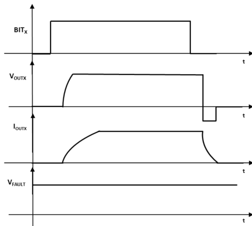
Figure 18. Switching on light inductive load
