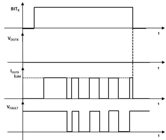
Figure 21. Switching on short-circuit (with OVT)
