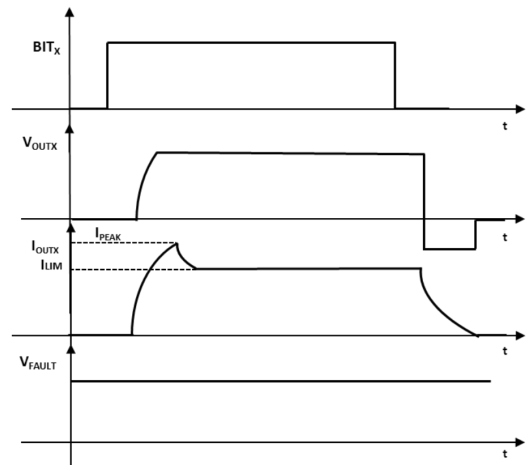
Figure 19. Switching on heavy inductive load
