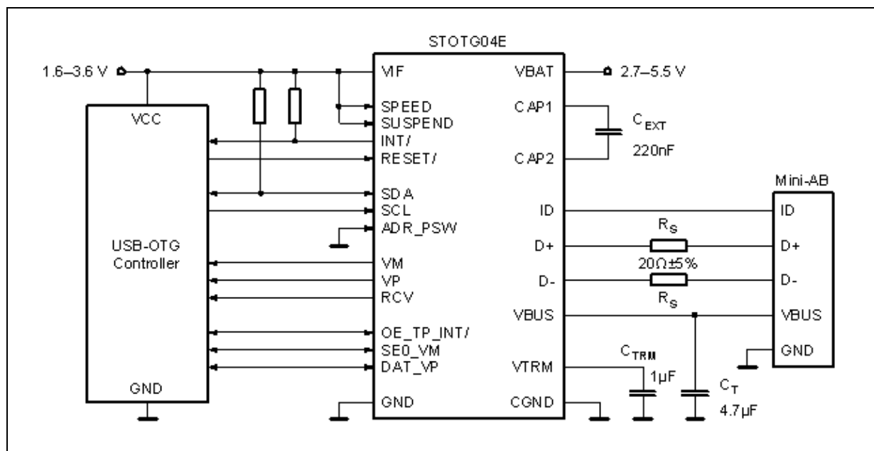
Figure 2. Functional diagram
