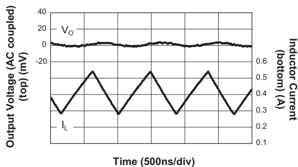
Output Ripple
