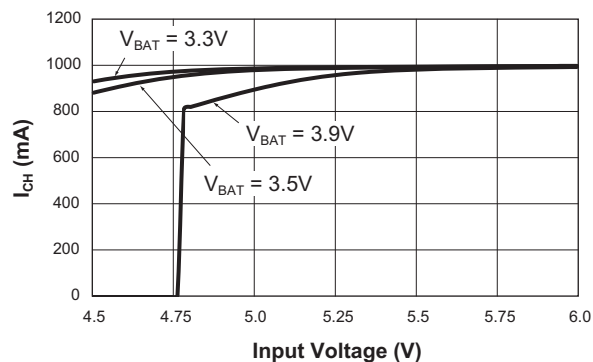
Constant Charging Current vs. Input Voltage (ADPSET = 8.06k \Omega )
