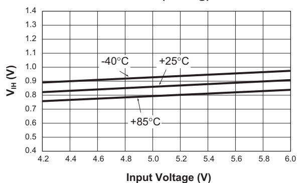
V_{IH} vs. Input Voltage EN Pin (Rising)
