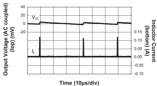
Output Ripple
