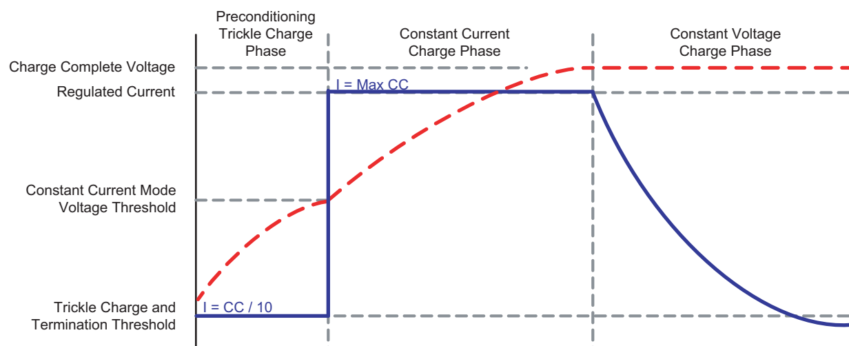
Figure 1: Typical Charge Profile.
