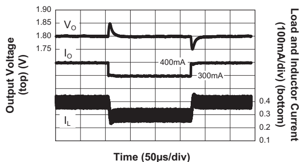
Load Transient Response (300mA to 400mA; V_{IN} = 3.6V ; V_{OUT} = 1.8V ; C_{OUT} = 4.7\mu F )
