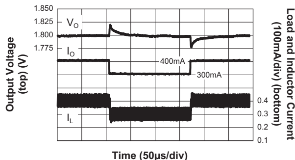
Load Transient Response (300mA to 400mA; V_{IN} = 3.6V ; V_{OUT} = 1.8V ; C_{OUT} = 10\mu F ; C_{FF} = 100pF )
