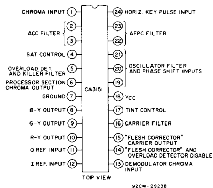
TERMINAL DIAGRAM
