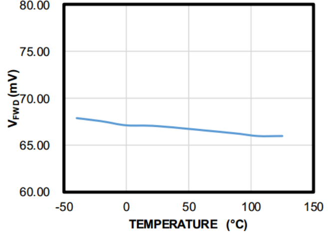
V FWD vs. Temperature
