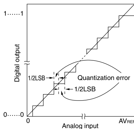
Figure 10-14. Quantization Error
