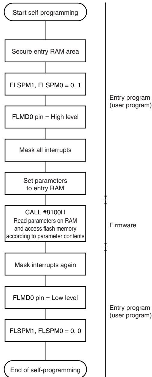
Figure 21-17. Self-Programming Procedure
