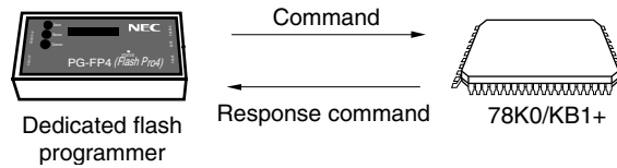
Figure 21-16. Communication Commands
