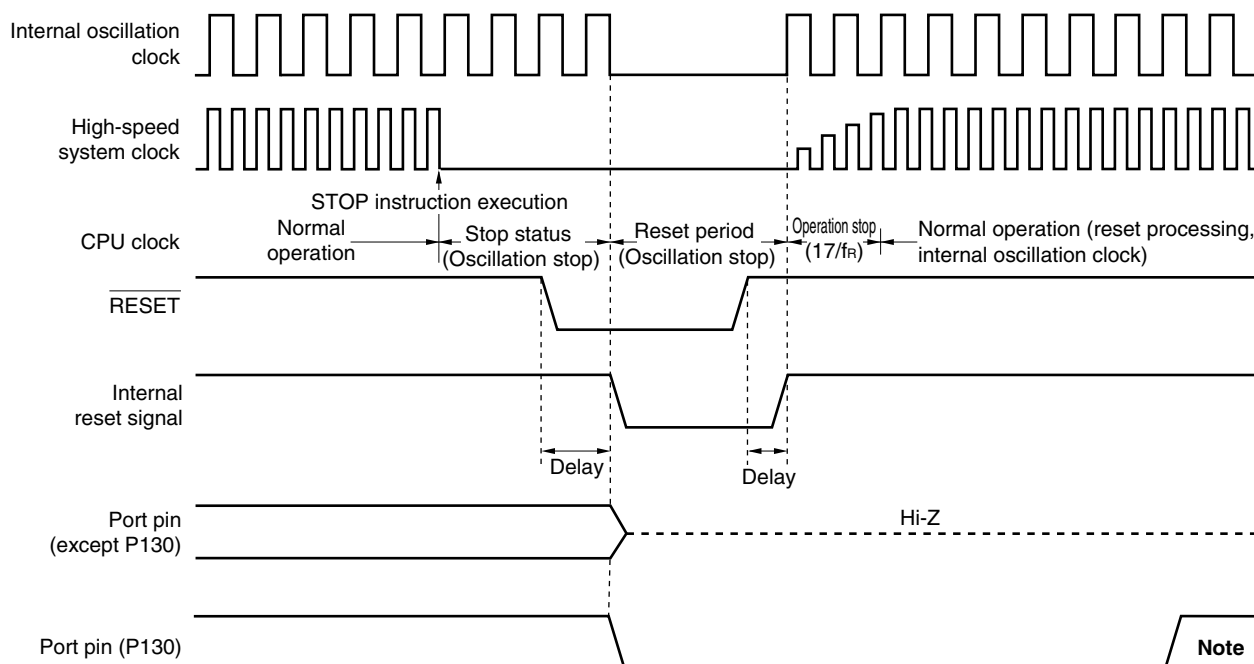
Figure 16-4. Timing of Reset in STOP Mode by RESET Input
