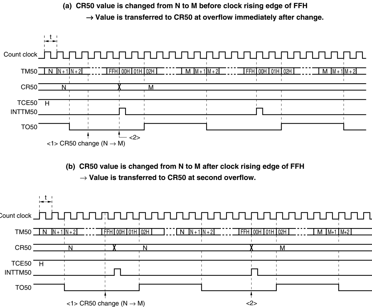
Figure 7-11. Timing of Operation with CR50 Changed
