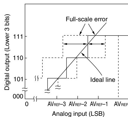
Figure 10-16. Full-Scale Error
