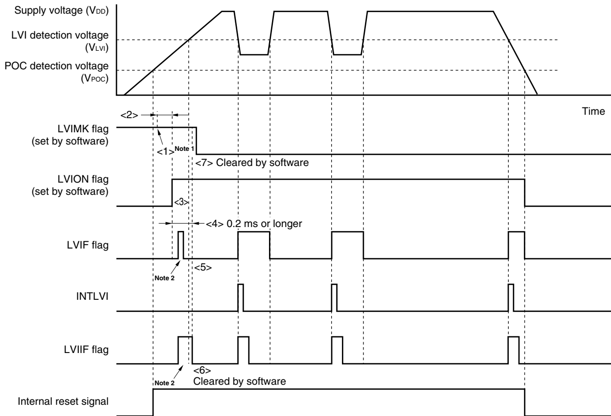
Figure 19-5. Timing of Low-Voltage Detector Interrupt Signal Generation
