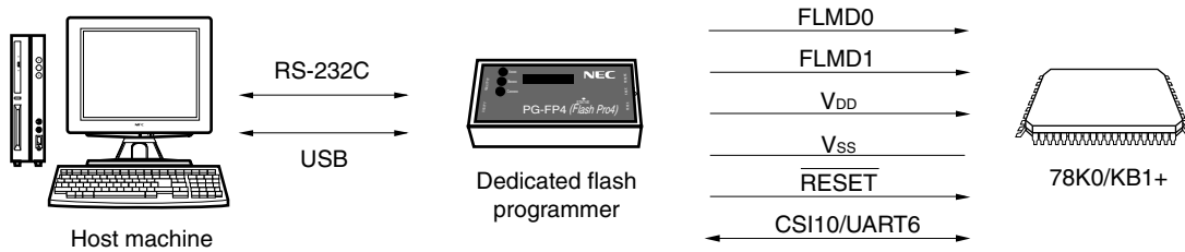
Figure 21-5. Environment for Writing Program to Flash Memory
