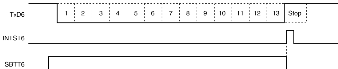
Figure 12-22. SBF Transmission
