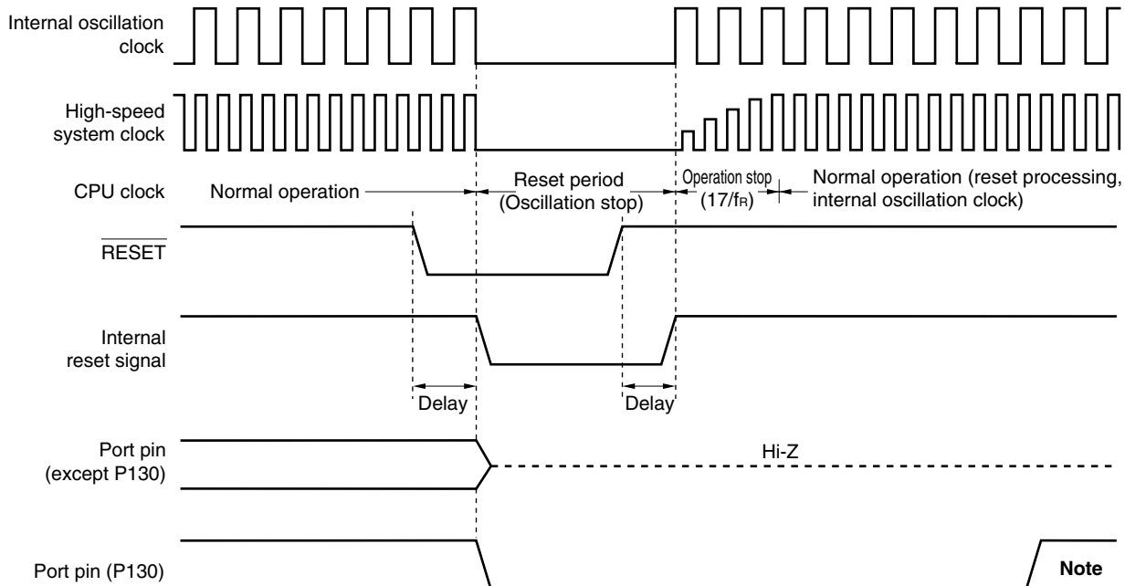
Figure 16-2. Timing of Reset by \overline{\text{RESET}} Input
