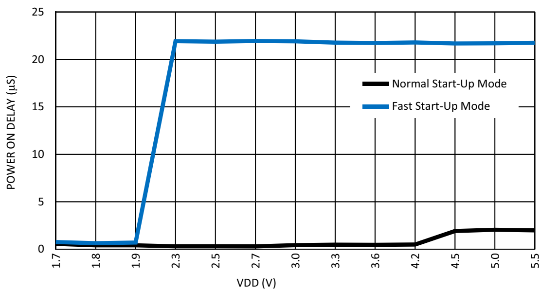
Figure 70. RC Oscillator Maximum Power On Delay vs. V_{DD} at 85°C, OSC0 = 25 kHz
