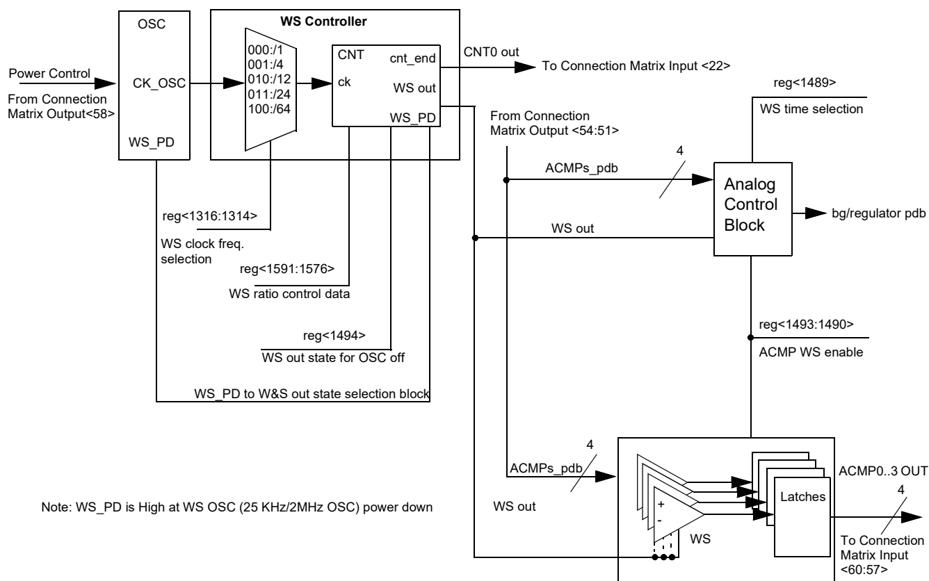
Figure 49. WS controller
