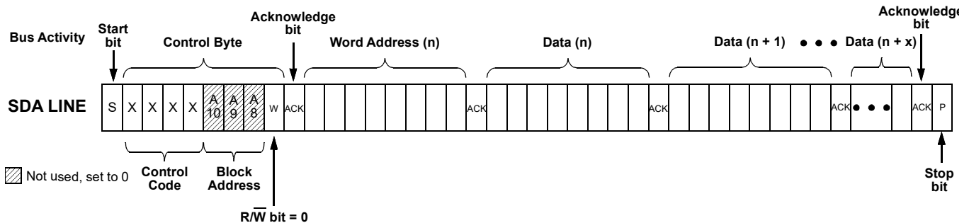
Figure 102. Sequential Write Command, R/\bar{W} = 0
