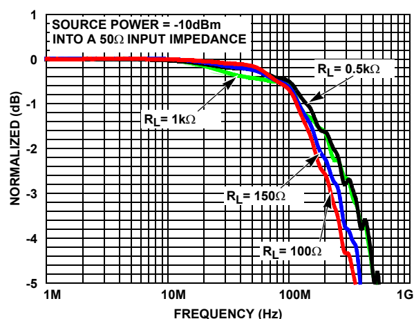
FIGURE 2. GAIN vs FREQUENCY vs R_L
