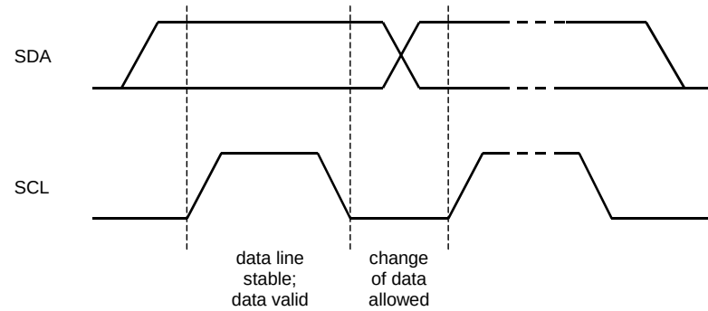
Figure 64. Bit Transfer (I 2 C Bus)
