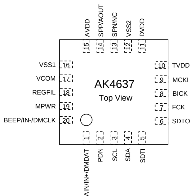
Figure 2. Pin Layout
