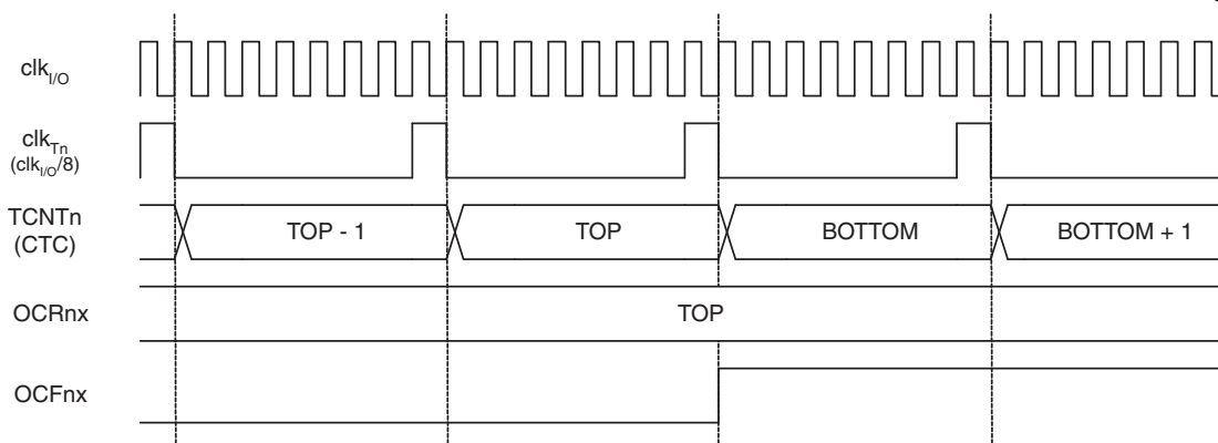
Figure 11-11. Timer/Counter Timing Diagram, Clear Timer on Compare Match mode, with Prescaler ( f_{\text{clk\_I/O}}/8 )
