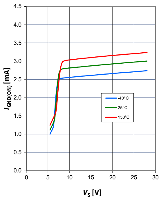
GND current when IN and DEN are biased to 5.5 V, I_{GND(ON)} = f(V_S, T_J)
