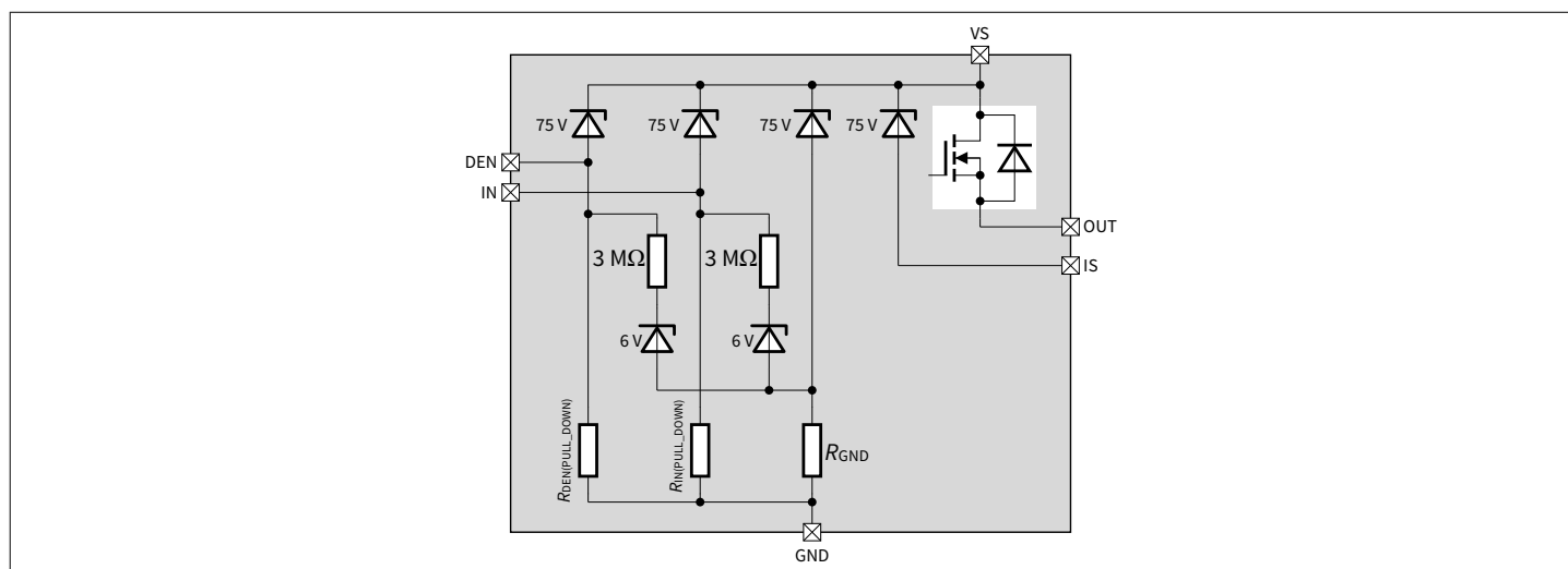
Figure 3 Internal diode diagram
