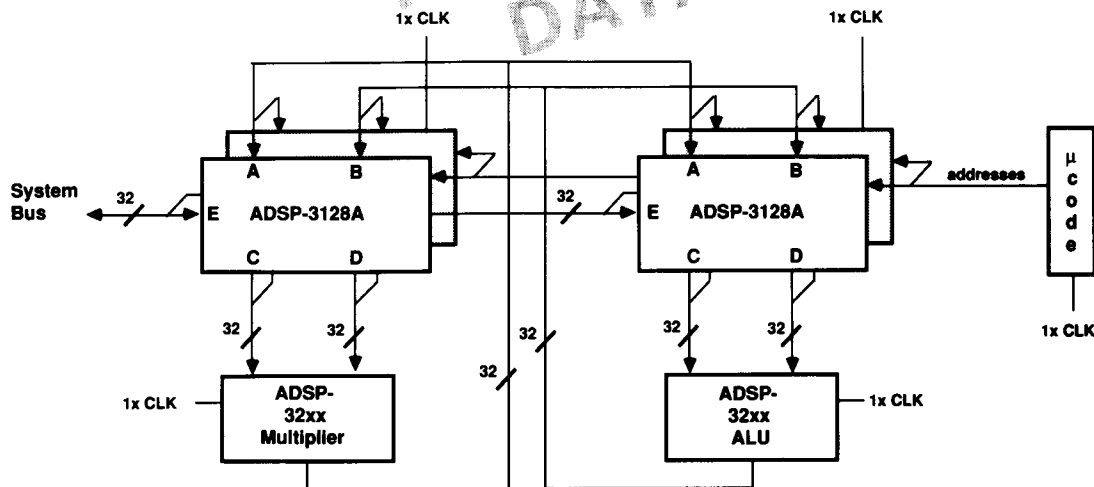
Figure 15. ADSP-3128A Seven-Port Double-Precision Application with ADSP-32XX
