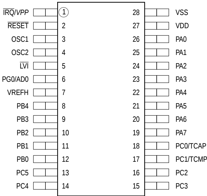
Figure 3 28-pin SOIC pinout
