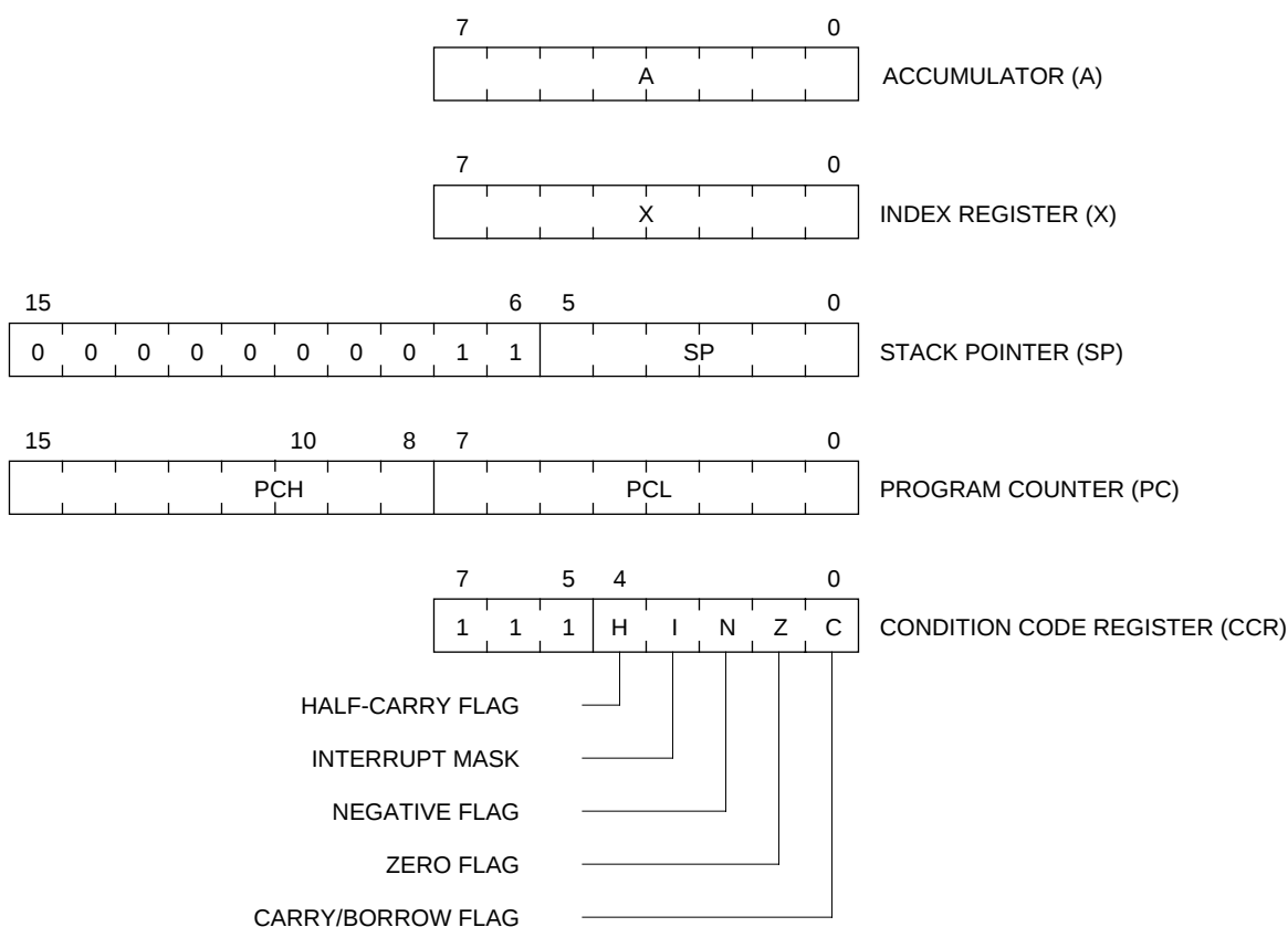
Figure 23 Programming Model
