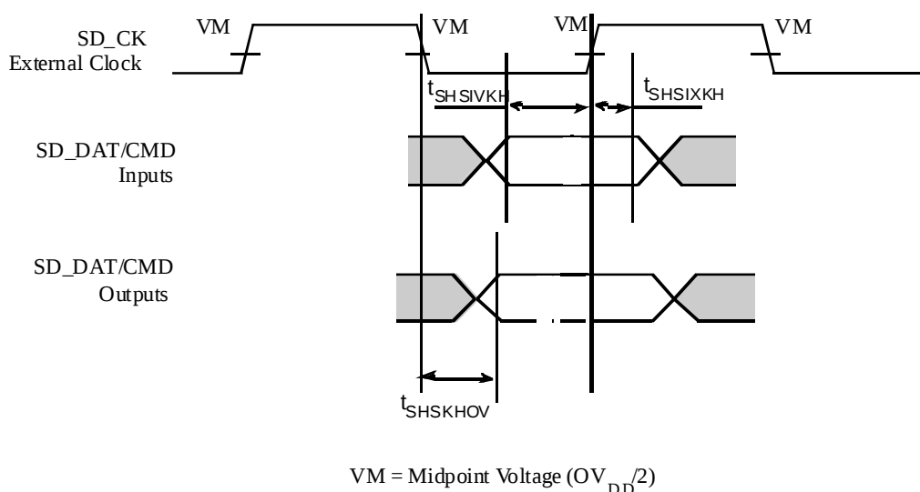
Figure 35. eSDHC Data and Command Input/Output Timing Diagram Referenced to Clock
