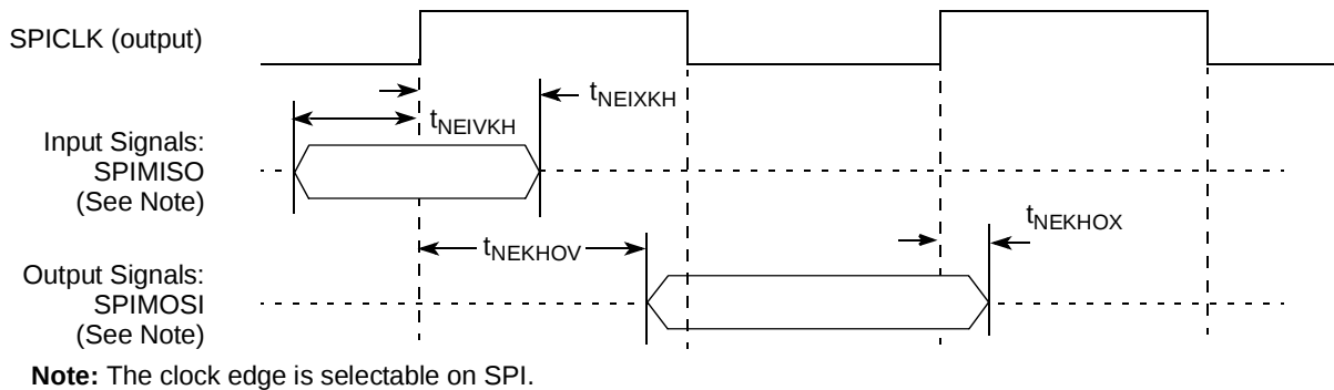
Figure 66. SPI AC Timing in Slave Mode (External Clock) Diagram
