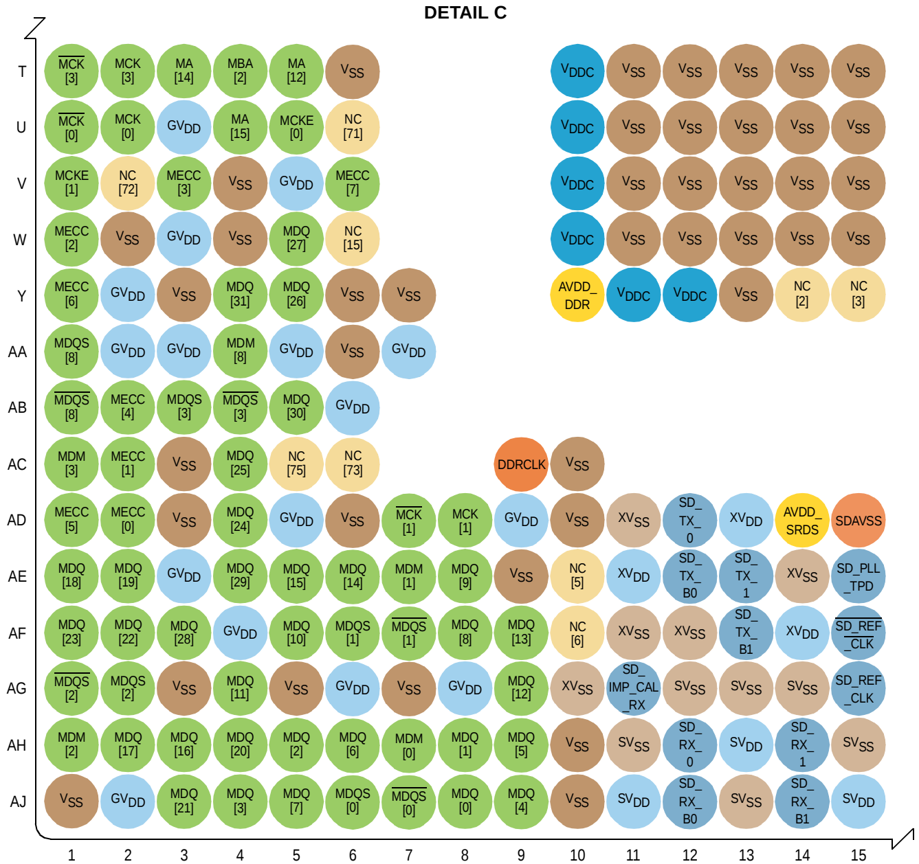
Figure 5. P1021 Detail C Ballmap
