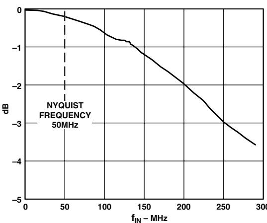
TPC 10. Frequency Response
