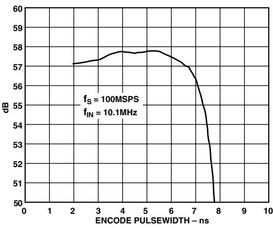
TPC 9. SNR vs. Clock Pulsewidth ( t_{EH} )
