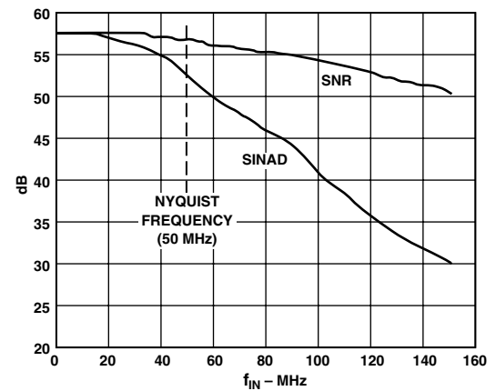
TPC 5. SNR vs. f_{IN} ; f_S = 100 MSPS
