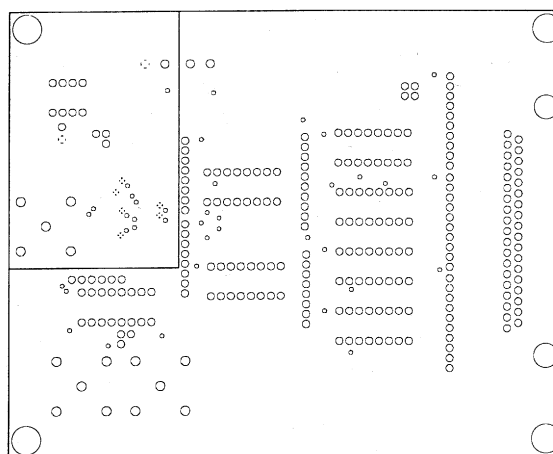
Figure 18. Analog/Digital Split Power Plane
