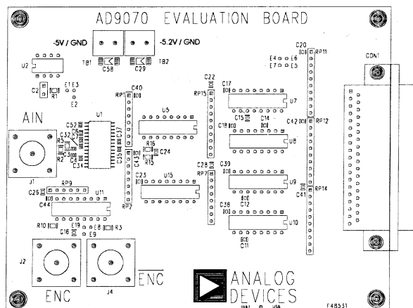
Figure 15. Component Side
