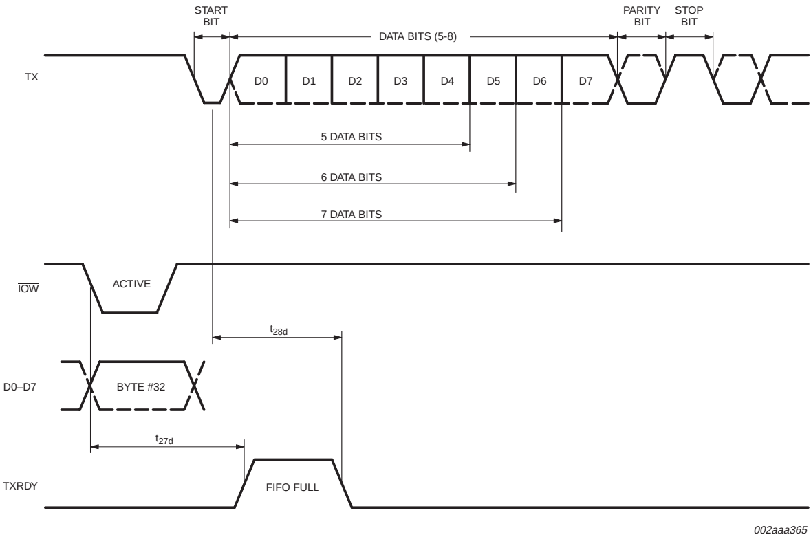
Fig 14. Transmit ready timing in FIFO mode (DMA mode '1').
