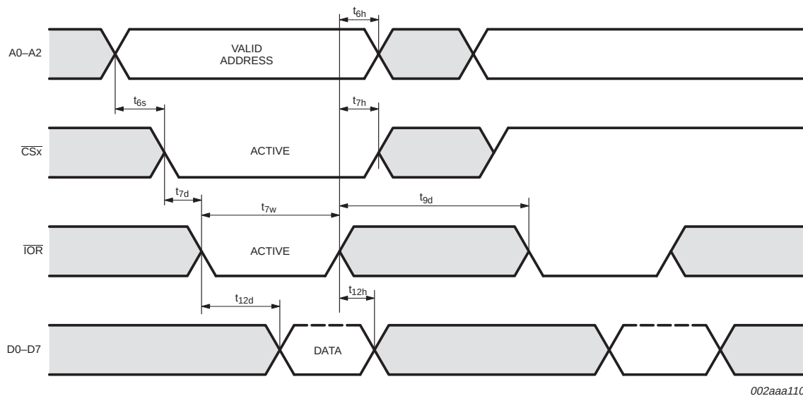
Fig 6. General read timing.
