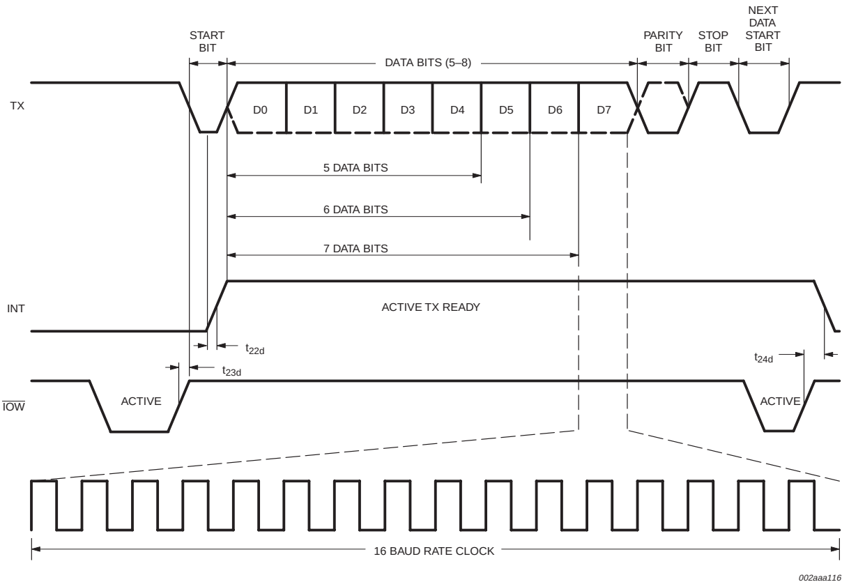
Fig 12. Transmit timing.
