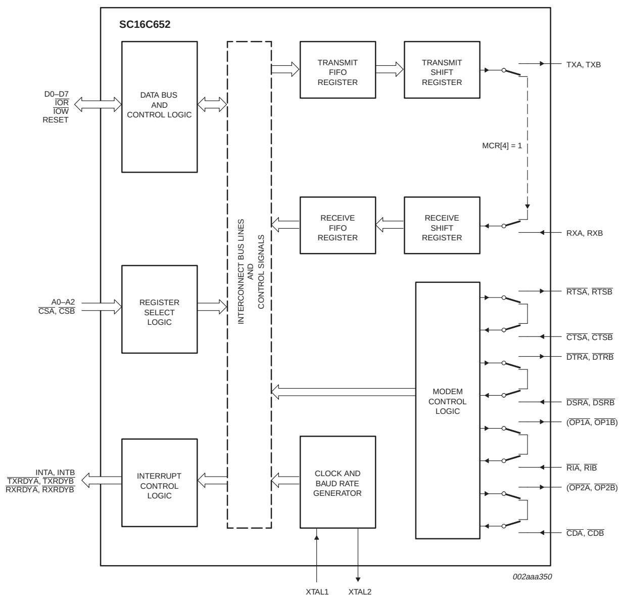
Fig 4. Internal loop-back mode diagram.
