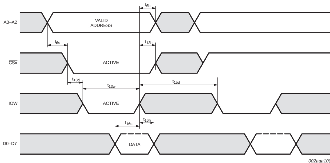
Fig 5. General write timing.
