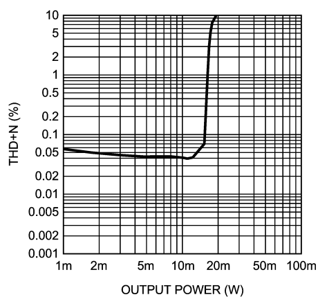
Headphone THD+N vs Output Power AV_{DD} = 3.3V , OCL 1.2V, 0dB AUX f_{OUT} = 1kHz , 32\Omega
