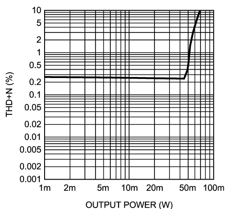
Headphone THD+N vs Output Power AV_{DD} = 3.3V , OCL 1.5V, 12dB AUX f_{OUT} = 1kHz , 16\Omega
