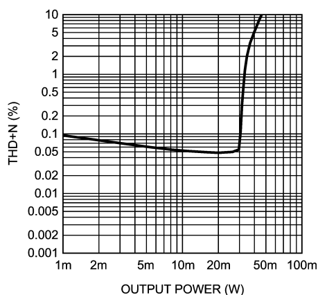
Headphone THD+N vs Output Power AV_{DD} = 3.3V , OCL 1.2V, 12dB AUX f_{OUT} = 1kHz , 16\Omega
