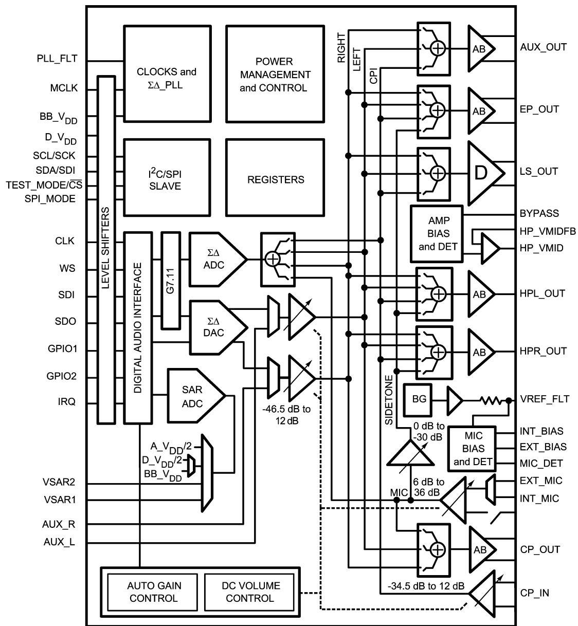
FIGURE 1. Conceptual Schematic
