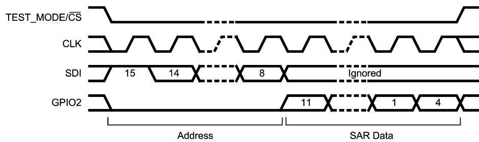
FIGURE 4. SPI Read Transaction
