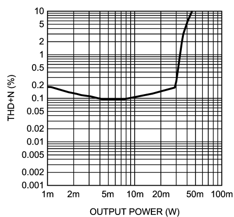
Headphone THD+N vs Output Power AV_{DD} = 3.3V , OCL 1.2V, 12dB DAC f_{OUT} = 1kHz , 16\Omega
