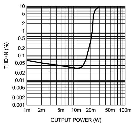
Headphone THD+N vs Output Power AV_{DD} = 3.3V , OCL 1.5V, 0dB AUX f_{OUT} = 1kHz , 32\Omega
