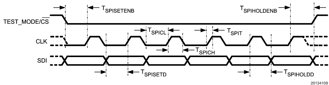
FIGURE 5. SPI Timing
