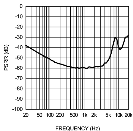
Loudspeaker PSRR vs Frequency AV_{DD} = 5V , 0dB AUX (AUX inputs terminated)
