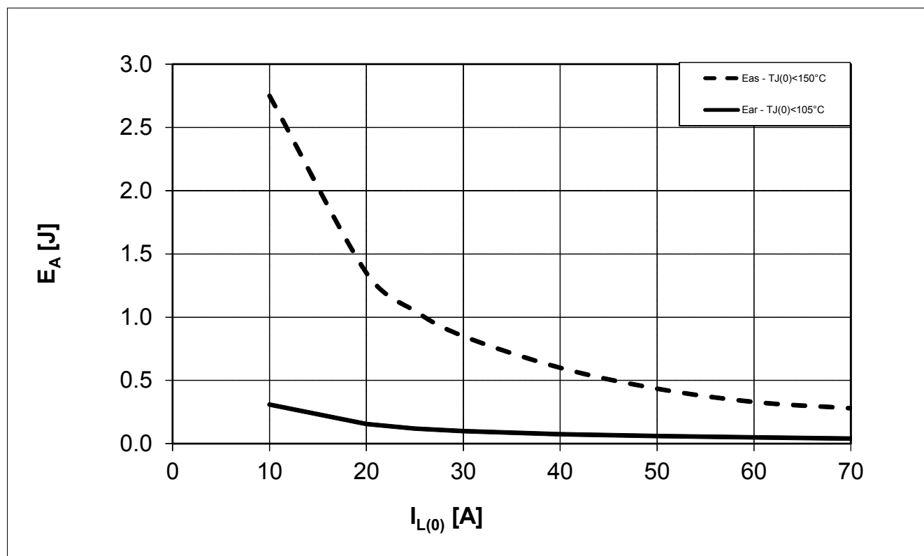
Figure 5 Maximum Energy Dissipation for Inductive Switch OFF, E_A vs. I_L at V_S = 13.5 V
