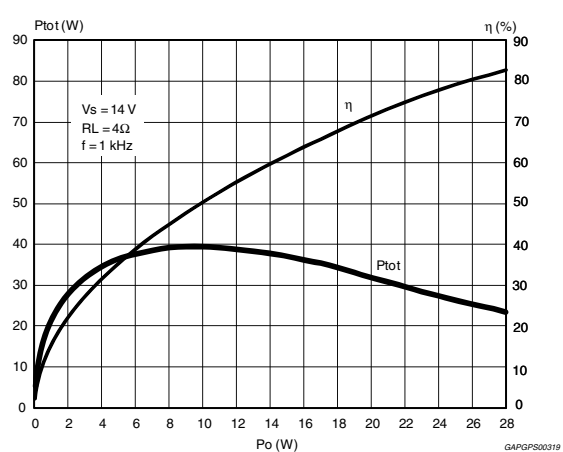
Figure 21. Total power dissipation and efficiency vs. output power (4 \Omega , STD, Sine)
