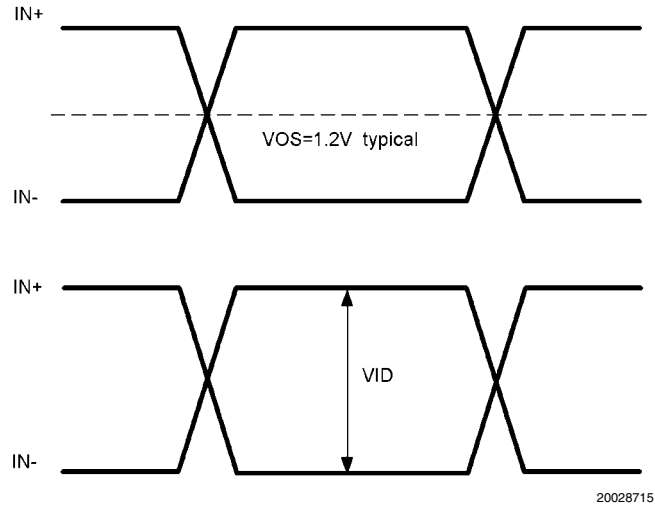
FIGURE 5. LVDS Signals
