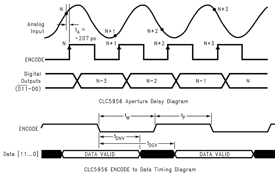
Timing Diagram
