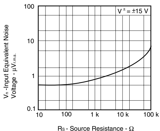
INPUT EQUIVALENT NOISE VOLTAGE (FLAT+JIS A)
