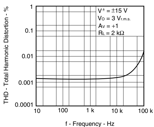
TOTAL HARMONIC DISTORTION
