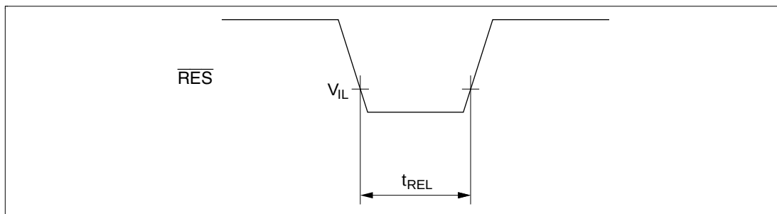
Figure 14.2 \overline{\text{RES}} Low Width Timing
