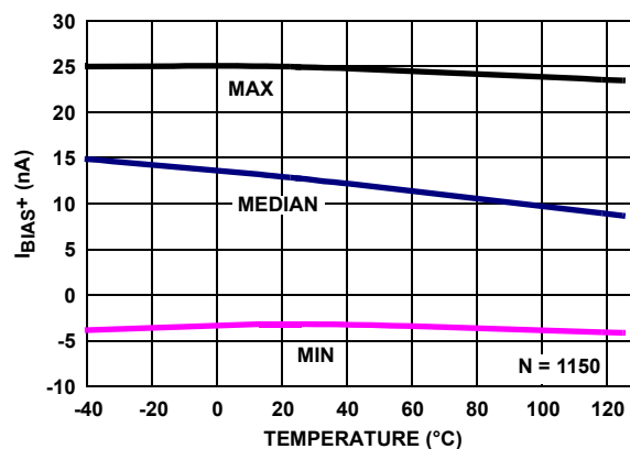
FIGURE 26. I_{BIAS+} vs TEMPERATURE, V_+ , V_- = \pm 2.5V
