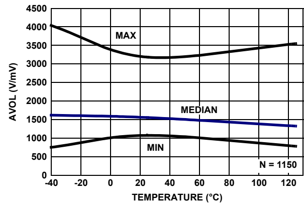
FIGURE 34. AVOL vs TEMPERATURE, V_+ , V_- = \pm 2.5V , V_O = -2V TO +2V , R_L = 100k
