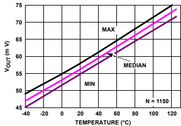
FIGURE 37. V_{OUT} LOW vs TEMPERATURE, V_+ = 5V , V_- = \pm 2.5V , R_L = 1k
