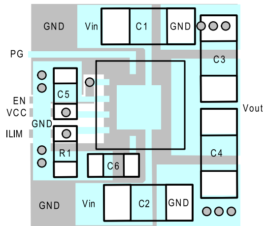
Figure 5: Recommended Layout
