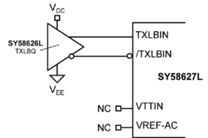
Figure 6f. TXLBIN Interface (AC-Coupled)
