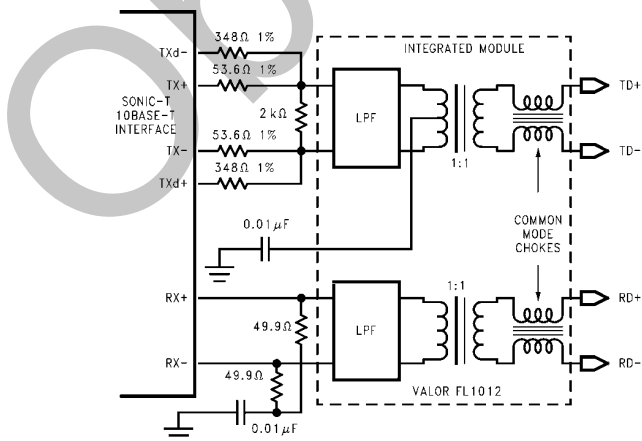
FIGURE 8-6. External Circuitry to Connect the SONIC-T to Twisted Pair Cable
