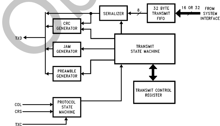
FIGURE 3-7. MAC Transmitter
