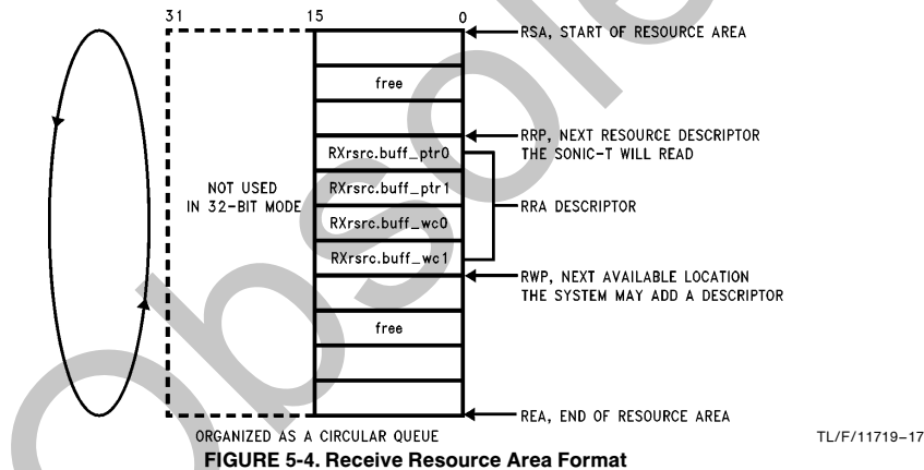
FIGURE 5-4. Receive Resource Area Format
