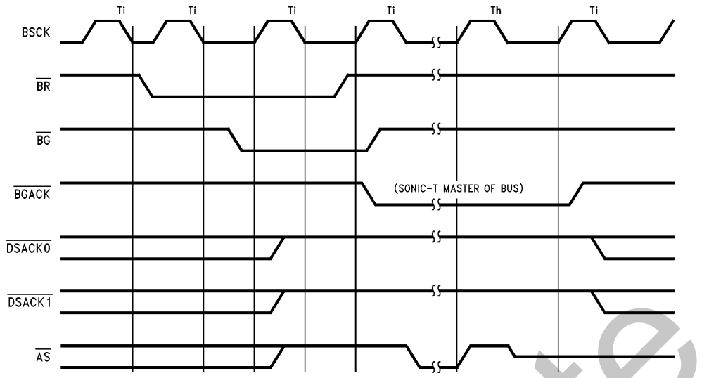
FIGURE 7-4. Bus Request Timing (BMODE = 1)
