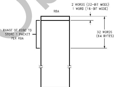
FIGURE 5-11. Setting EOBC for Single Packet RBA
