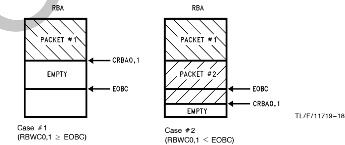
FIGURE 5-5. Receive Buffer Area
