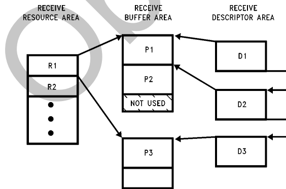
FIGURE 5-3. Overview of Receive Buffer Management
