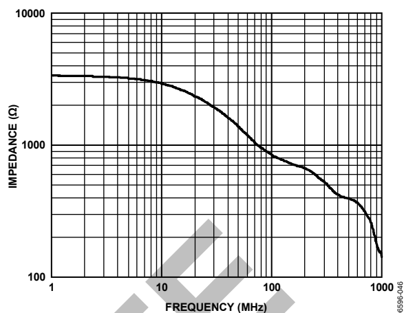
Figure 35. Input Impedance
