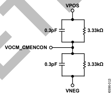
Figure 14. VOCM_CMENCON Input (See Also ESD Protection Map, Figure 19)
