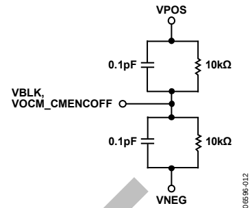
Figure 13. VBLK and VOCM_CMENCOFF Inputs (See Also ESD Protection Map, Figure 19)
