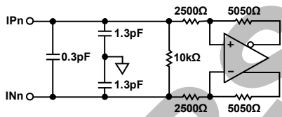
Figure 10. Receiver Differential (See Also ESD Protection Map, Figure 19)
