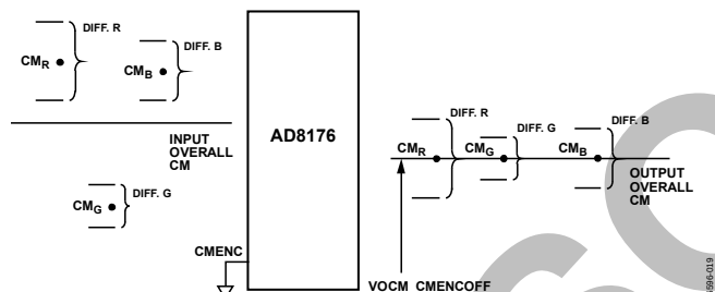
Figure 46. AD8176 in Middle of Cat-5 Run Application, CM Encoding Off (Note that in this application, the H and V outputs, though asserted, are not used.)
