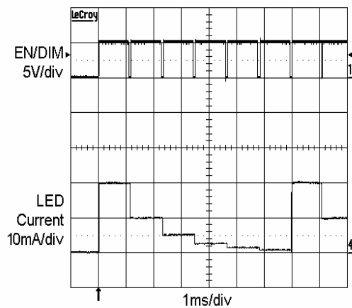
Dimming Waveform
