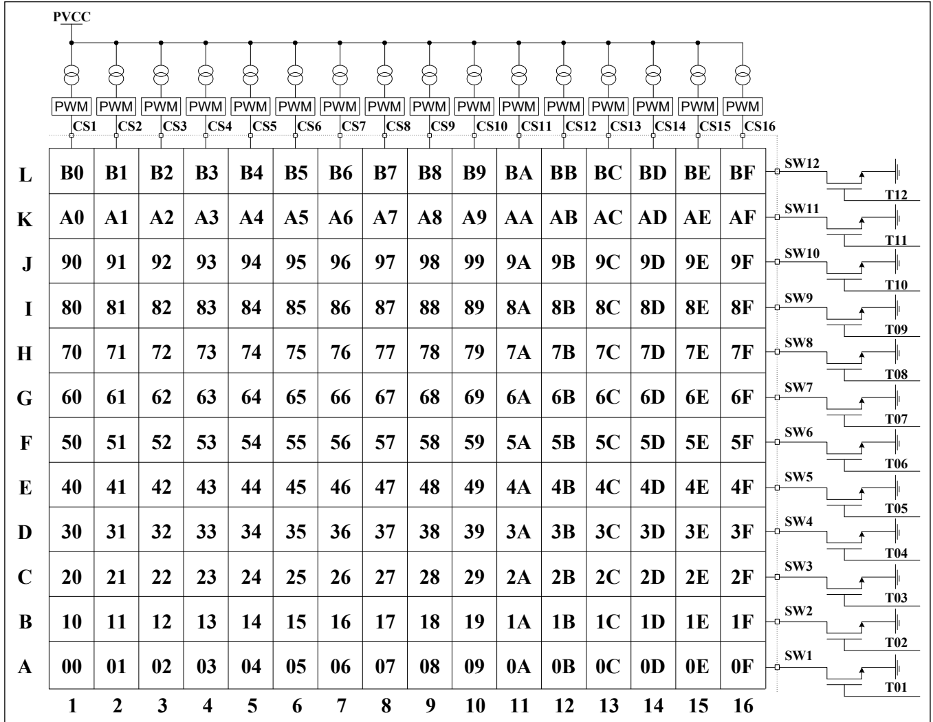
Figure 9 PWM Register
