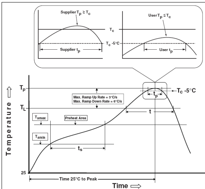
Figure 19 Classification Profile
