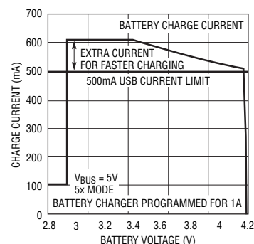
Battery Charge Current vs Battery Voltage (LTC3586)
