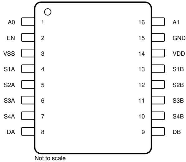
Figure 6-3. PW Package 16-Pin TSSOP Top View
