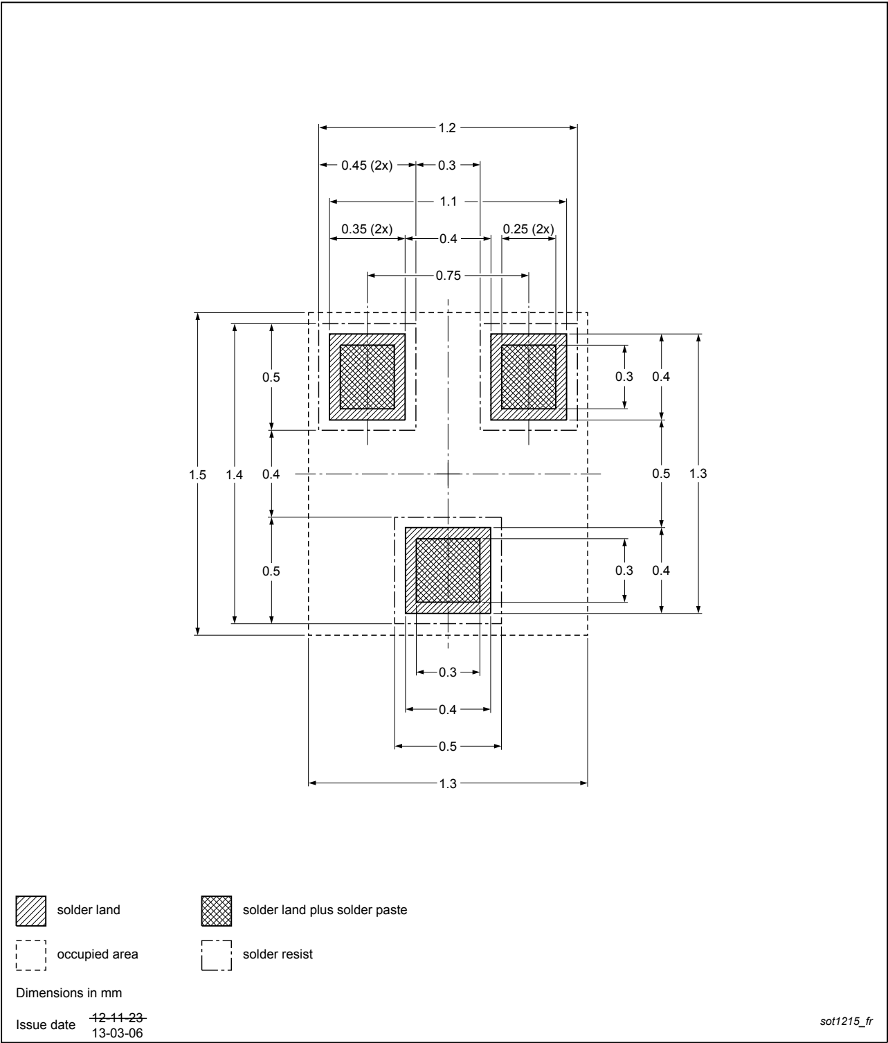
Fig. 12. Reflow soldering footprint for DFN1010D-3 (SOT1215)
