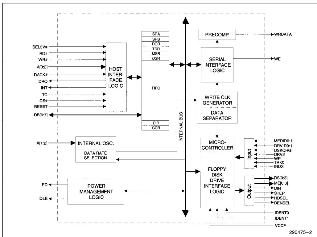
Figure 1-1. 82078 Block Diagram
