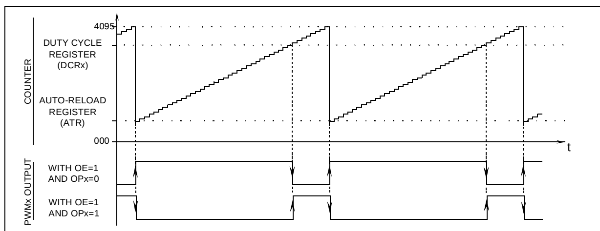
Figure 36. PWM Function
