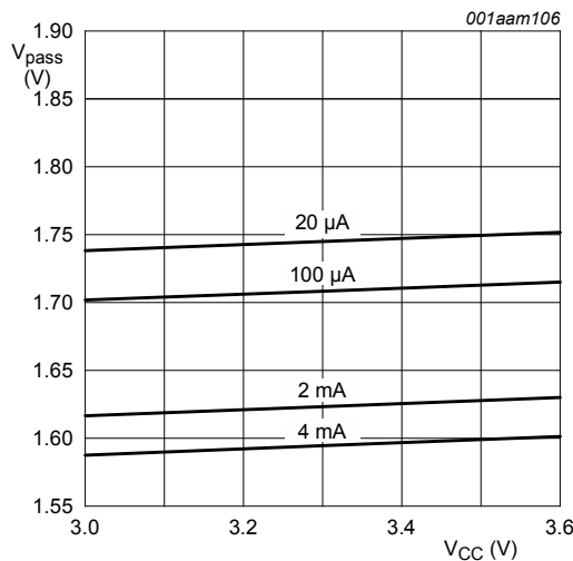
Fig. 11. Pass voltage versus supply voltage; T_{\text{amb}} = -40\text{ }^{\circ}\text{C} (typical)
