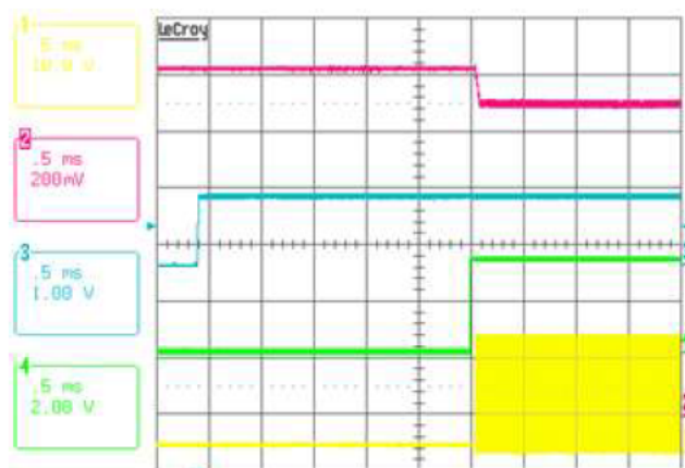
FIGURE 37. VR2 PRE-CHARGED START UP, V_{IN} = 19V , V_{ID} = 1.1V , V_{PRE-CHARGE VOLTAGE} = 1.3V , CH1: PHASE1G, CH2: VR2 V_O , CH3: VR_ON, CH4: PGOOD
