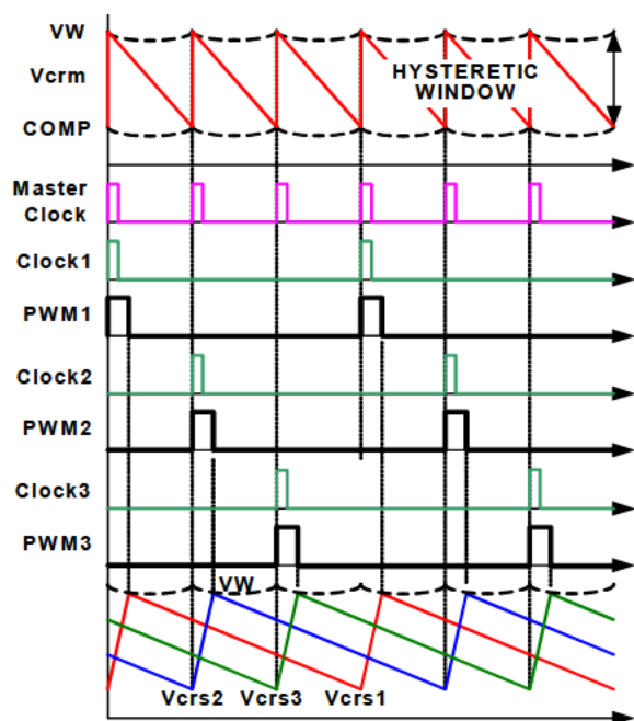
FIGURE 5. R3™ MODULATOR OPERATION PRINCIPLES IN STEADY STATE
