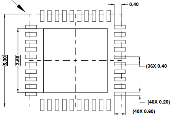
PACKAGE OUTLINE
