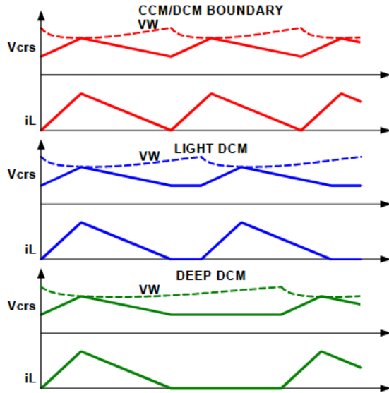
FIGURE 8. PERIOD STRETCHING
