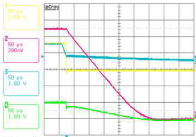
FIGURE 35. VR2 SHUT DOWN, V_{IN} = 12V , I_O = 5A , V_{ID} = 1.1V , CH1: PGOODG, CH2: VR2 V_O , CH3: VR_ON, CH4: COMPG
